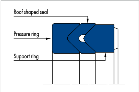
Merkel Chevron Seal Set EK, EKV
