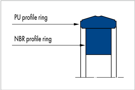
Merkel Compact Seal Simko 300
