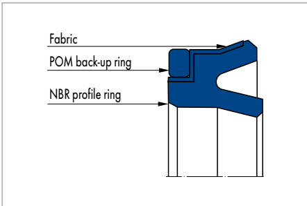
Merkel U-Ring NA 400
