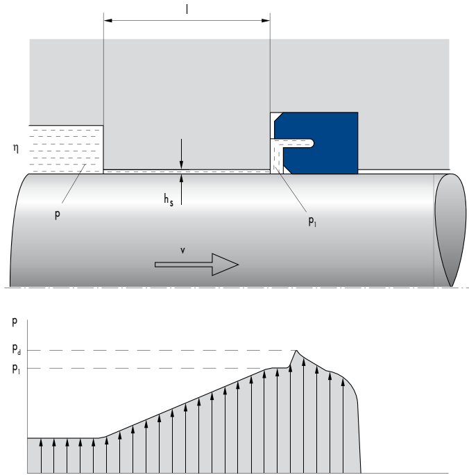
Fig. 17 Hydrodynamic drag pressure
