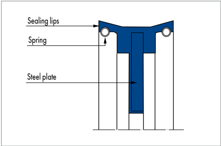
Merkel Complete Piston TDUOH
