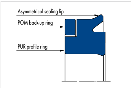
Merkel U-Ring T 18
