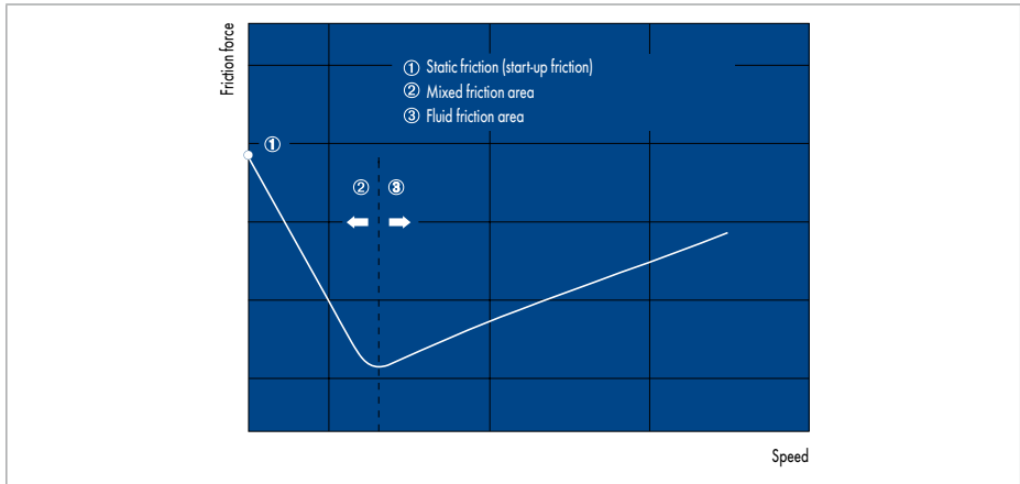
Fig. 16 Stribeck graph
