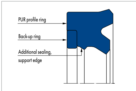
Merkel U-Ring TM 23
