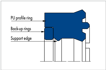
Merkel Compact Seal KI 320
