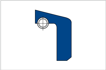
Merkel Cup Packing T with Spring
