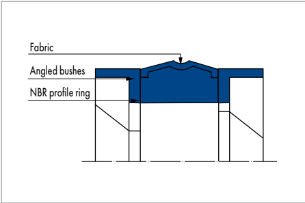
Merkel Compact Seal Simko 320 X2
