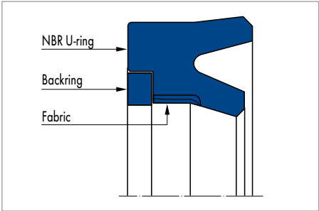
Merkel U-Ring Seal Set 0216
