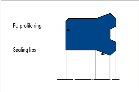
Merkel Compact Seal KI 310
