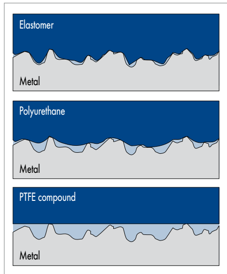
Fig. 33 Sealing edge in contact with counter surface
