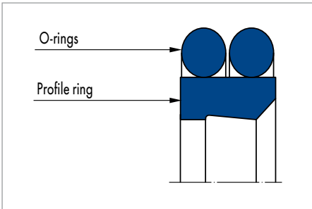
Merkel Double Wiper PT 1
