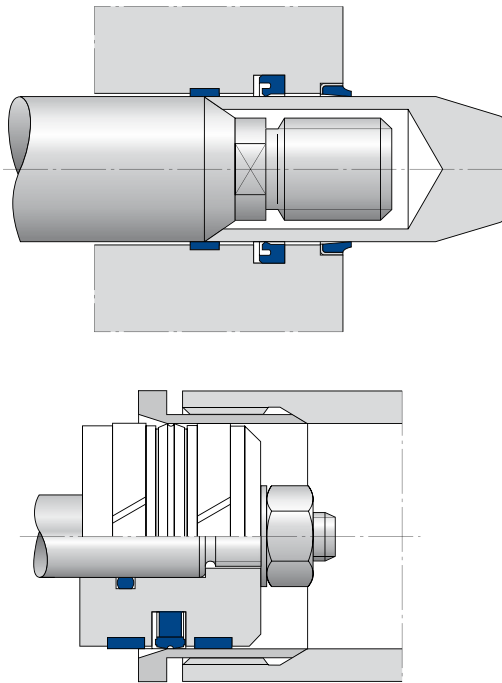
Fig. 37 Covering threads when mounting seals
