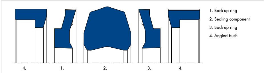
Fig. 52 Fitting of Merkel Compact Seal L 43
