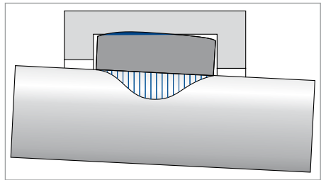
Merkel Guide Ring Guivex KBK: even distribution of stress
