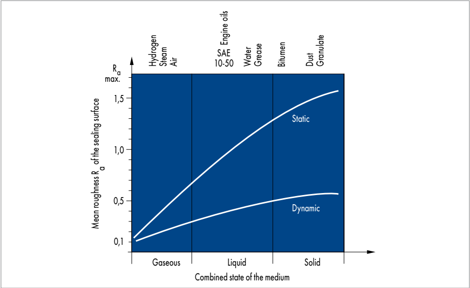
Surface recommendation for sealing surfaces
