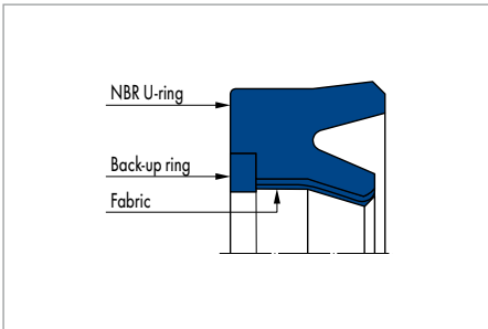
Merkel U-Ring Seal Set 0214
