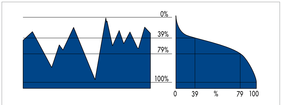
Fig. 29 Abbott graph
