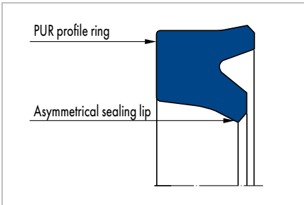
Merkel U-Ring T 20
