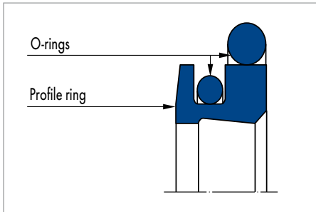
Merkel Double Wiper PT 2
