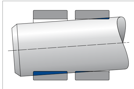
Fig. 12 Bilateral contact
