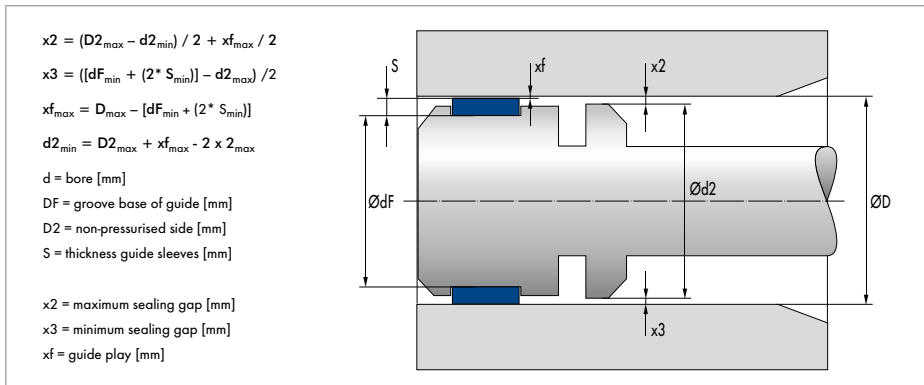
Fig. 23 Limit values of sealing gap of piston sealing system
