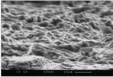
Fig. 27 Salt-bath-nitrated surface
