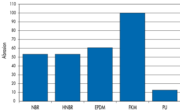
Fig. 35 Wear behaviour in comparison
