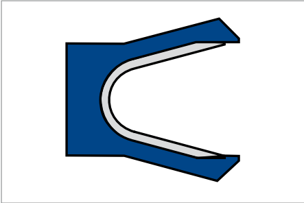
Forseal FOA made of PTFE
