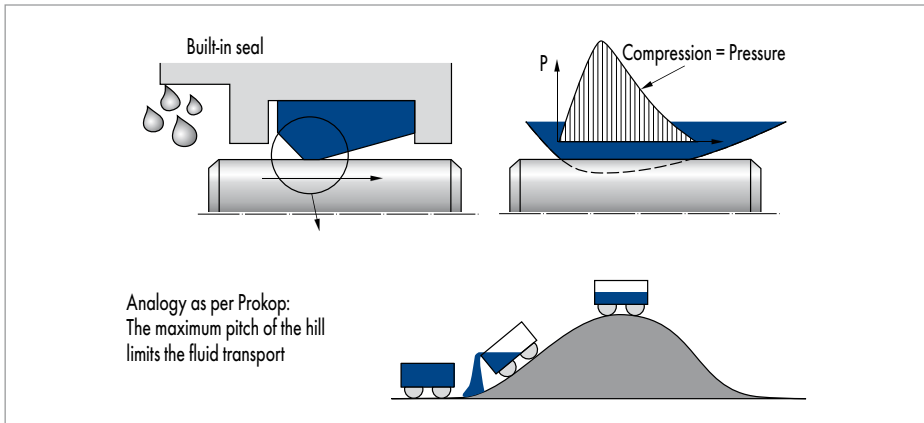
Fig. 5 Qualitative compression curve, single-acting rod seal
