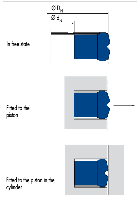
Fig. 3 Piston seal
