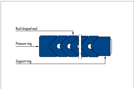
Merkel Chevron Seal Set ES, ESV
