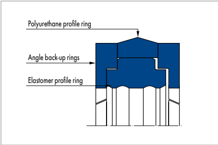
Merkel Compact Seal T 44
