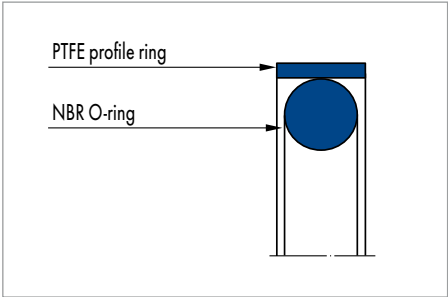
Merkel Compact Seal TFMA
