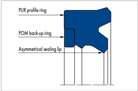
Merkel U-Ring T 23
