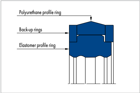
Merkel Compact Seal T 42
