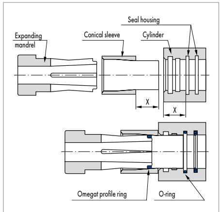
Fig. 51 Finished assembly tools (on enquiry)
