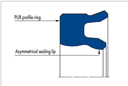
Merkel U-Ring TMP 20
