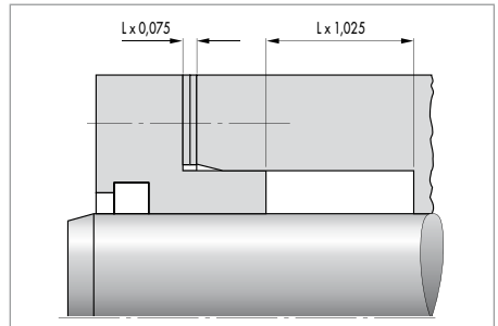
Fig. 54 DMS installation space example
