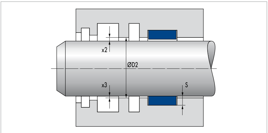
Fig. 14 Sealing gap
