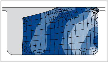
Cover Seal at 40 MPa operating pressure
