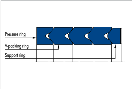
Merkel V-Packings V 1000
