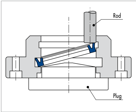
Fig. 41 Installation aid for rod seals
