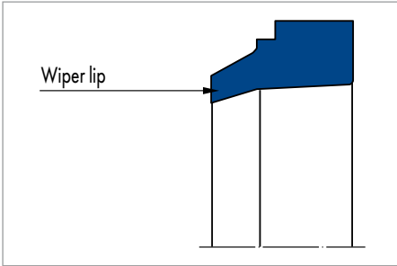
Merkel Wiper ASOB
