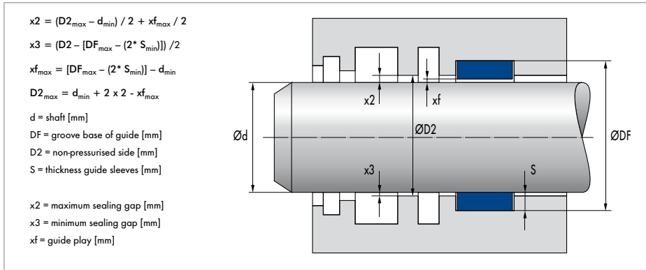
Fig. 22 Limit values of sealing gap of rod sealing system
