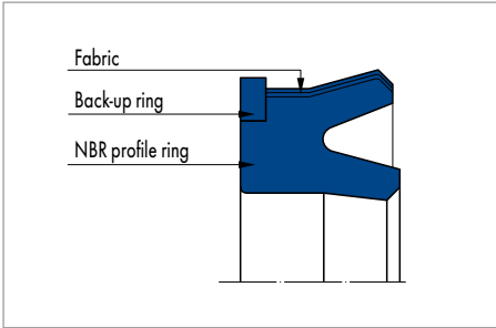
Merkel U-Ring Seal Set 0215
