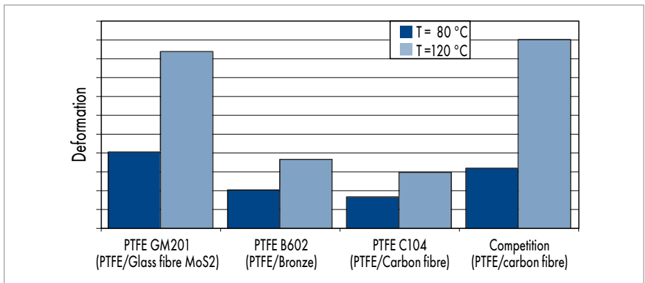
Fig. 34 Form stability of PTFE compounds in comparison
