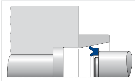
Fig. 42 Fitting of rod seals in divided housings
