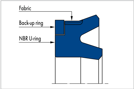
Merkel U-Ring Seal Set 0217
