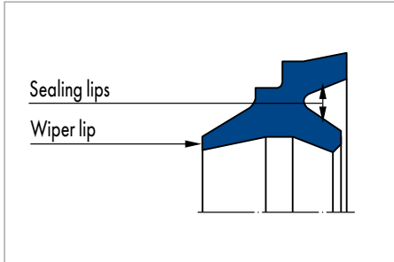
Merkel Double Wiper P 8
