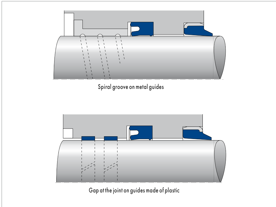
Fig. 19 Design measures for preventing drag pressure
