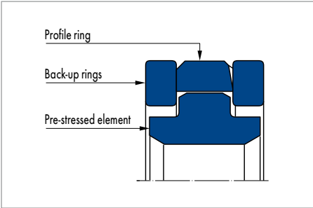
Merkel Compact Seal L 27
