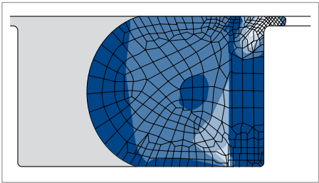
O-ring with PTFE back-up ring at 40 MPa operating pressure
