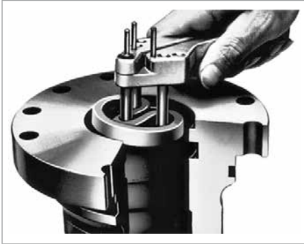
Fig. 39 Fitting tool I for rod seals
