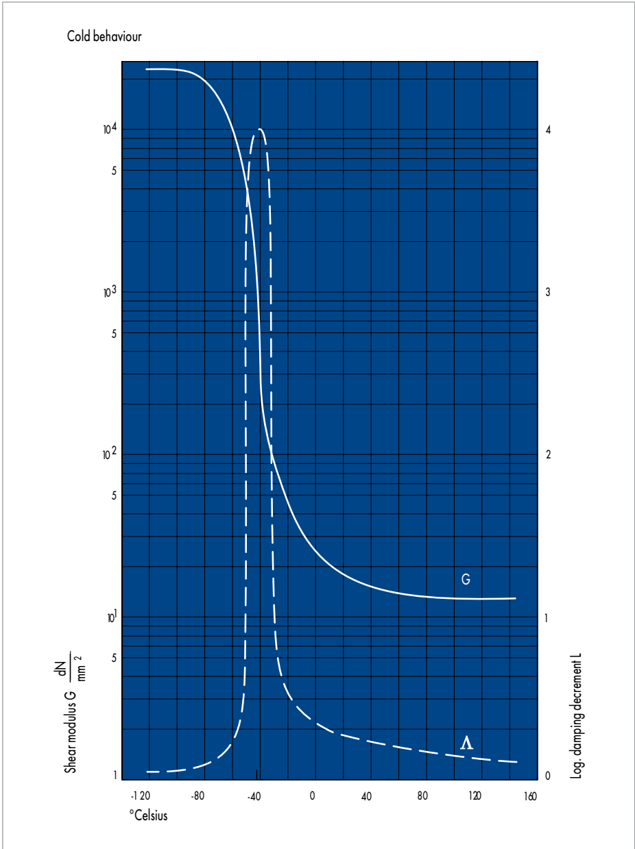
Fig. 20 Graph: torsion vibration test in accordance with DIN 53445; dynamic shear modulus G and logarithmic decrement \Lambda of a FST material based on CR
