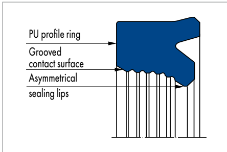
Merkel U-Ring LF 300
