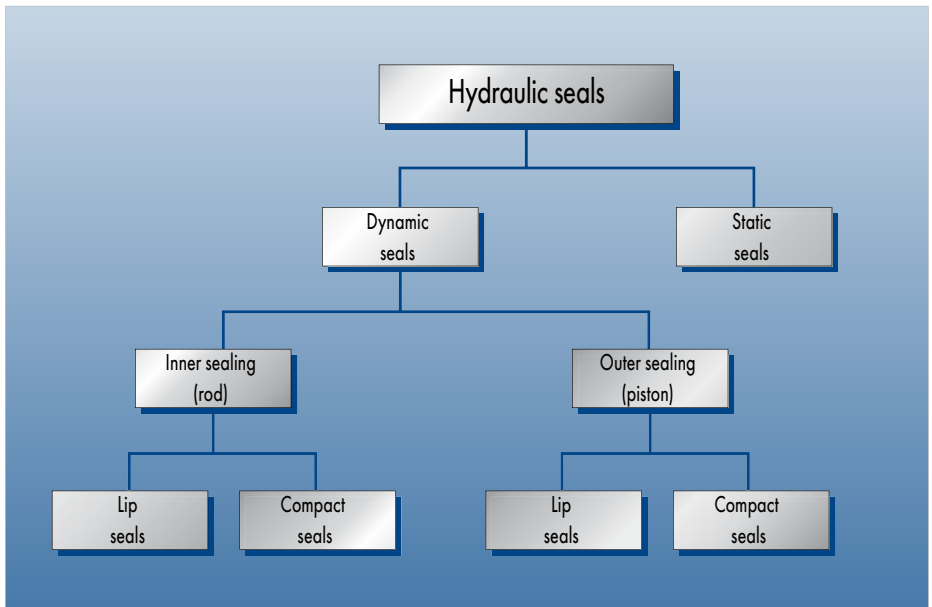
Fig. 1 Categorisation of hydraulic seals
