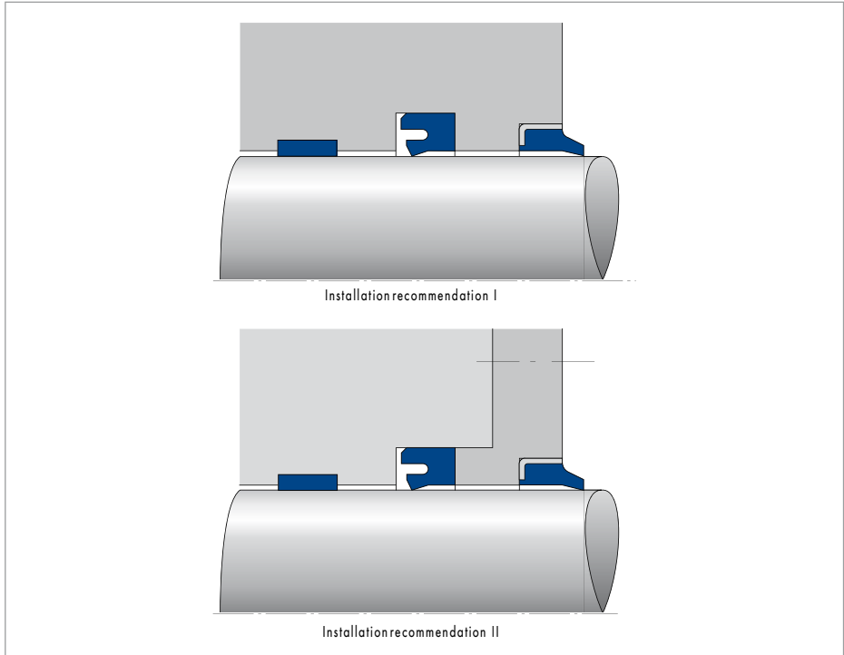
Fig. 38 Installation types of rod seals
