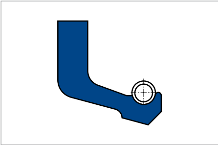
Merkel Hat Seal H with Spring
