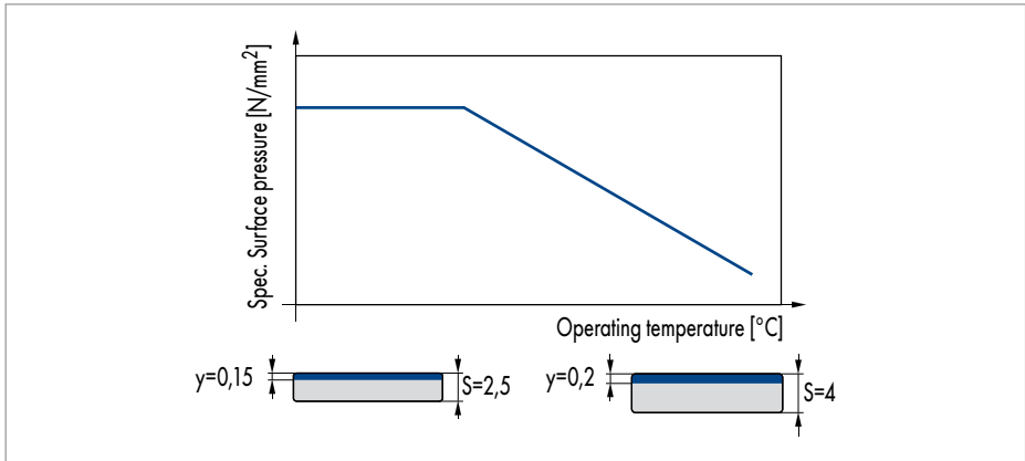
Fig. 13 Deflection at maximum surface pressure
