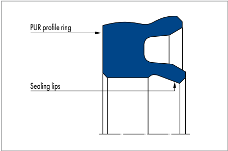
Merkel U-Ring TMP 21
