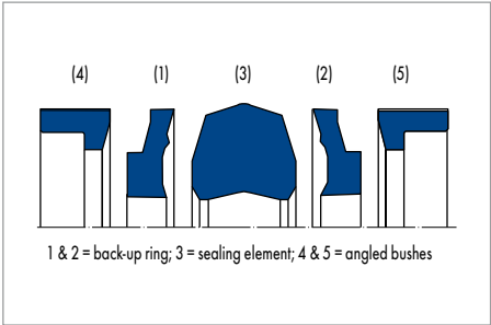
Merkel Compact Seal L 43
